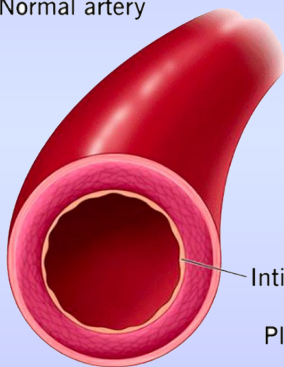
Normal artery
